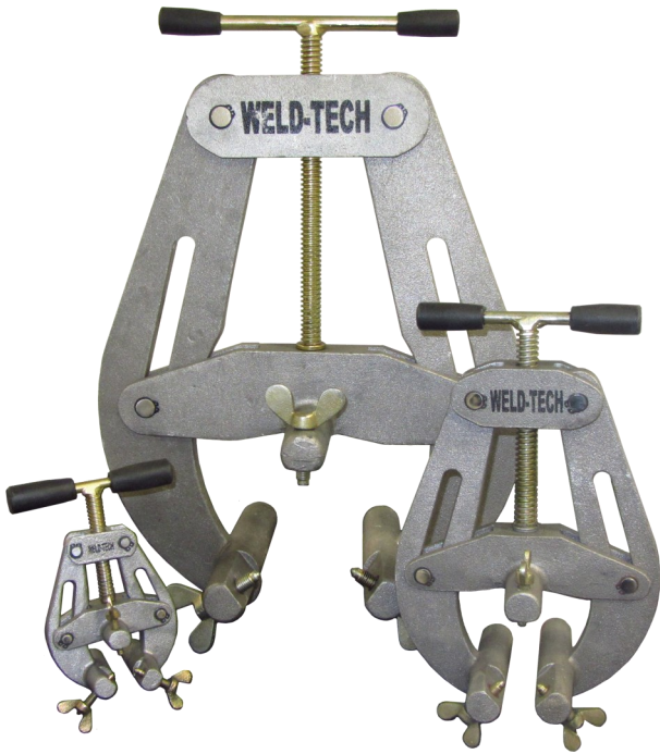
The Weld-Tech Family: 4 Clamps ranging from 1" through to 14"
